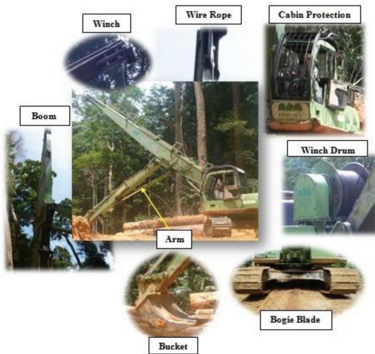
Fig.1: The RIMBAKA Timber Harvester R2020-A
